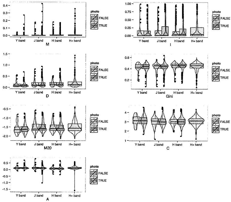
Figure 22: Comparison between two theories explaining inconsistency between the two methods we used.
