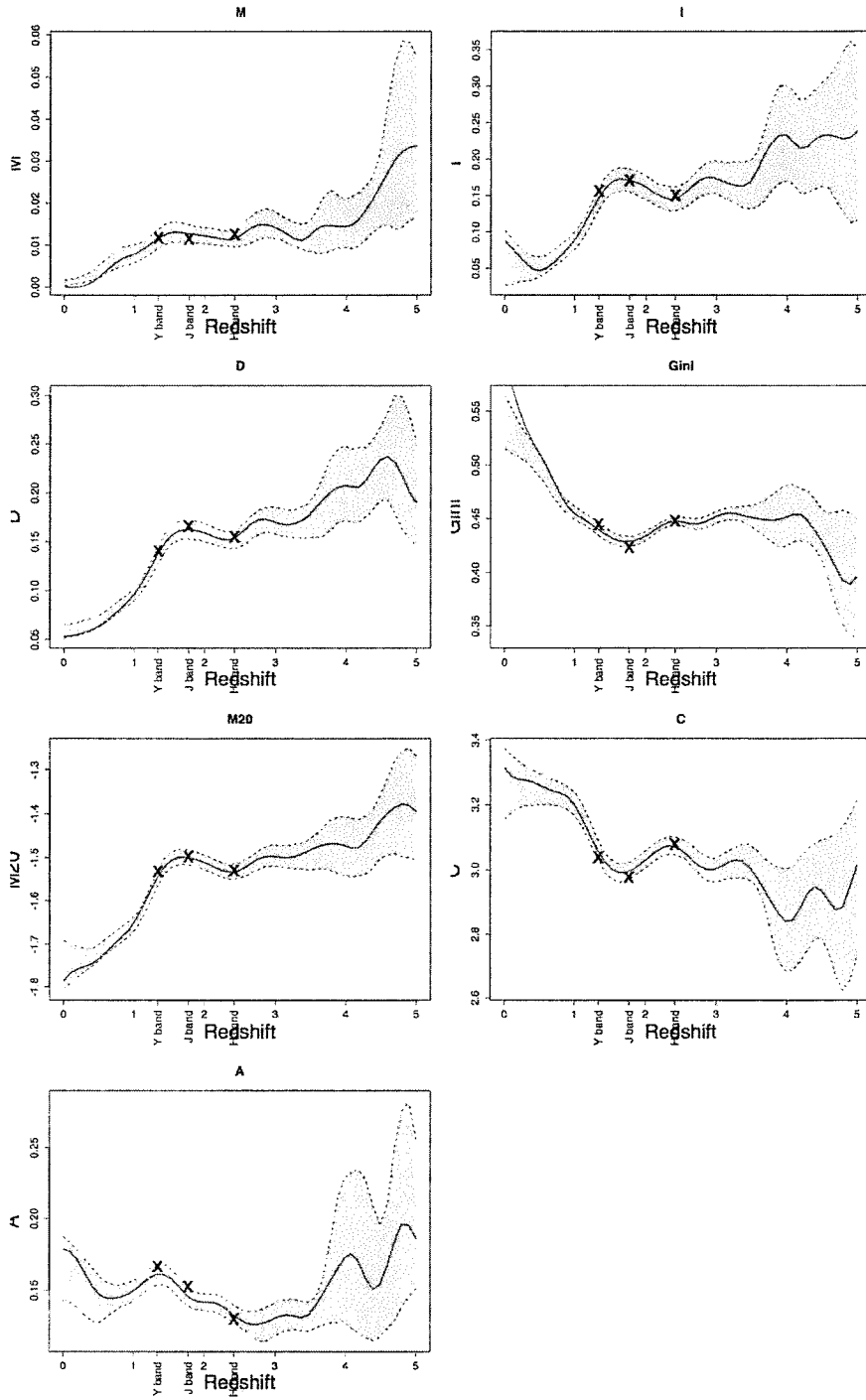
Figure 15: Same as Figure 13, for GOODS field.
