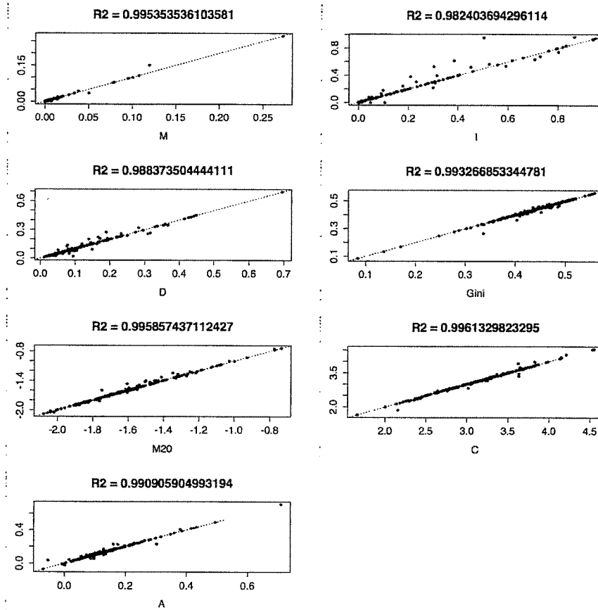
Figure 20: Comparing the weighted average from statistics taken in 3 filter bands to the true feature statistics taken in Y band for galaxies in Y band redshift range.
