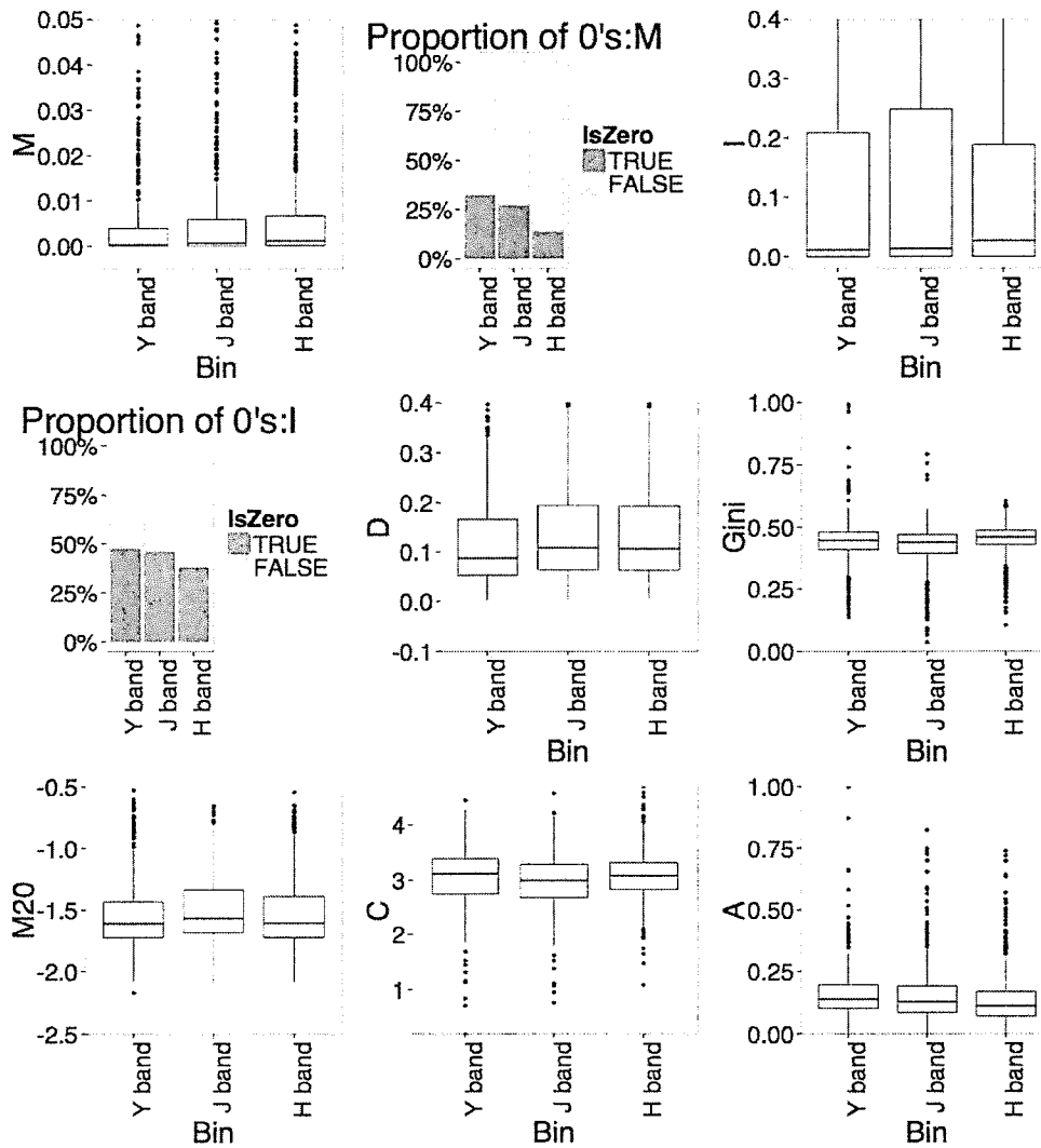
Figure 11: Same as Figure 10, for the GOODS field. We see slight differences in behavior of portion of zeroes in M and I, but the trend is still largely consistent with Figure 10.
