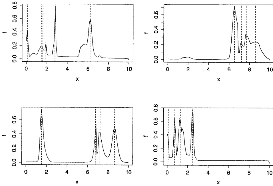
Figure 8: These are some multimodal galaxies identified in the procedure described above. Most of the spurious modes are eliminated. For example, in the top right figure, the small peak in density around Z = 2 is correctly ignore. Also, in the bottom right figure, the peak very close to the third mode is also correctly ignored.
