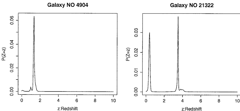
Figure 4: The redshift of most galaxies have only one mode, yet some galaxies do exhibit bimodality or other irregular shapes in the distribution of their redshift estimates.
