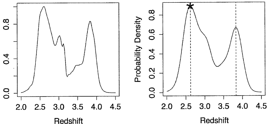
Figure 7: Noise leads to many spurious peaks in the density function for redshift of galaxy number 42. The smoothed version of the density function, however, helps us easily identify the two significant modes at z = 2.62 and z = 3.83 .
