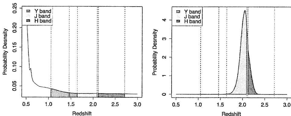
Figure 6: Illustration of mapping galaxies to redshift bins based on photometric redshift measurement. The curve is density function of redshift given by photometric redshift measurement, while shaded areas are probability of the redshift being in the redshift range of each filter band. Here the galaxy on the left is not mapped to any redshift bins while the galaxy on the right is mapped to the J band. We set the probability threshold at 0.8 here.
