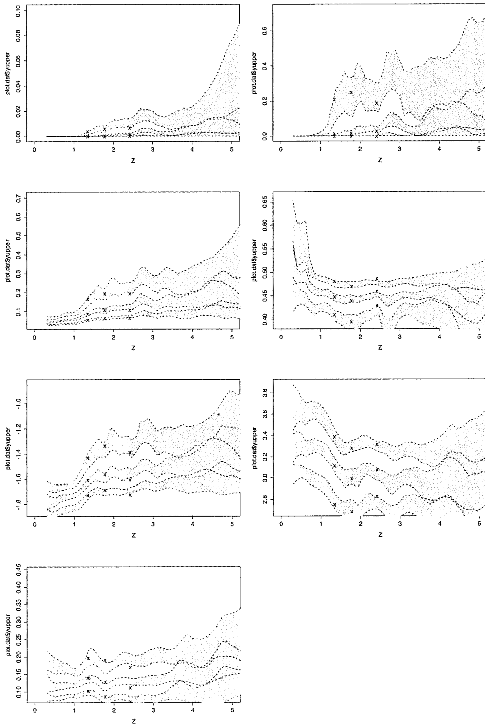
Figure 17: For each conditional \tau -quantile, we provide its corresponding interval estimate via design matrix bootstrap, resampling from the galaxy population of GOODS-N field 500 times.
