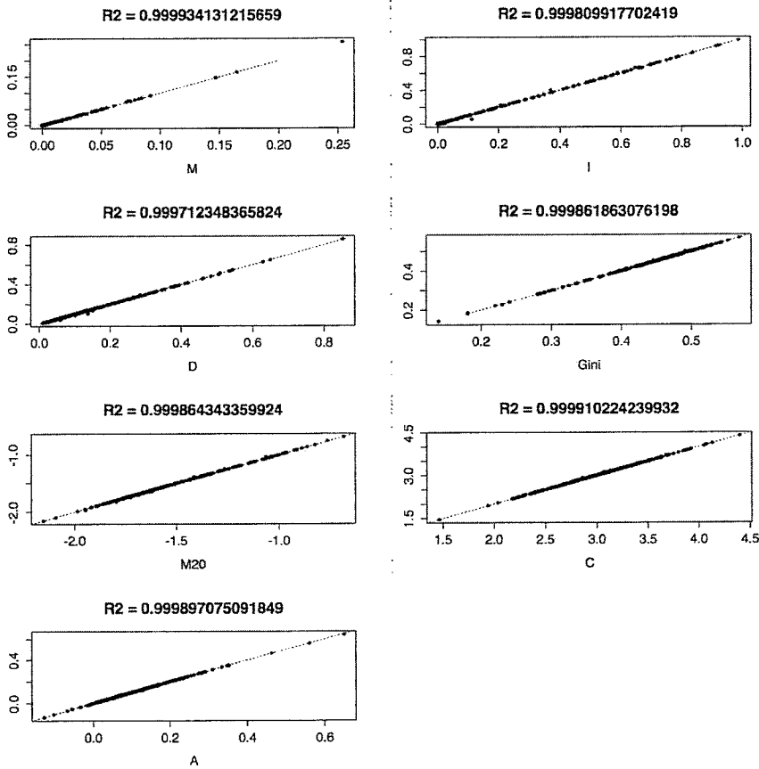
Figure 19: Comparing the weighted average from statistics taken in 3 filter bands to the true feature statistics taken in J band for galaxies in J band redshift range.
