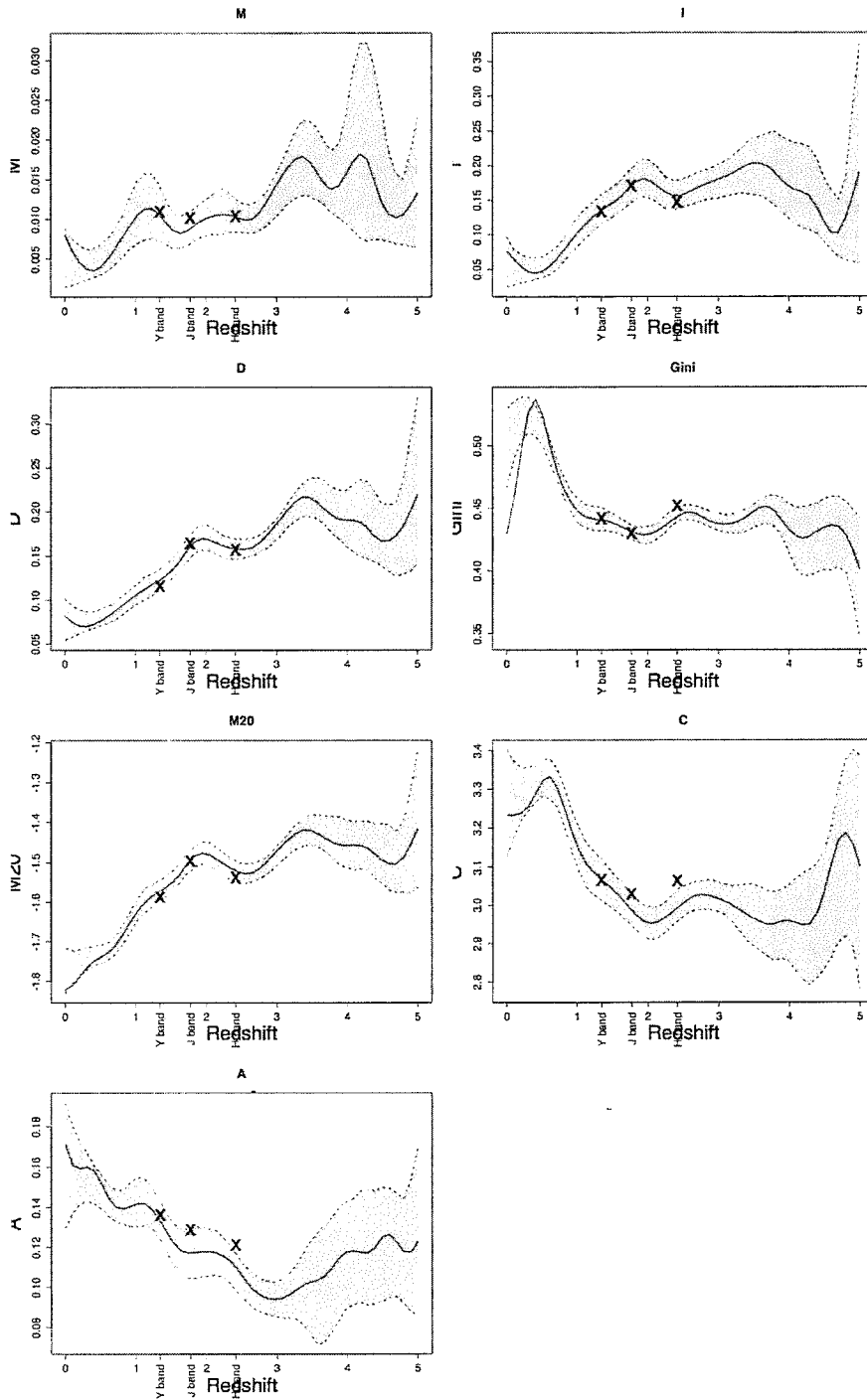
Figure 13: Comparison between the mean of each redshift bin and confidence band of the kernel regression using galaxies in the GOODSS field.
