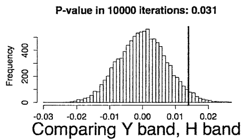
Figure 23: Bootstrap T test for C and A statistic in GOODSS field. P-values are not adjusted for multiple testing.
