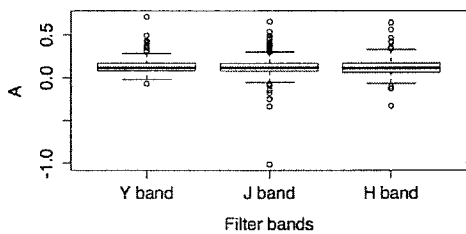
Figure 23: Bootstrap T test for C and A statistic in GOODSS field. P-values are not adjusted for multiple testing.
