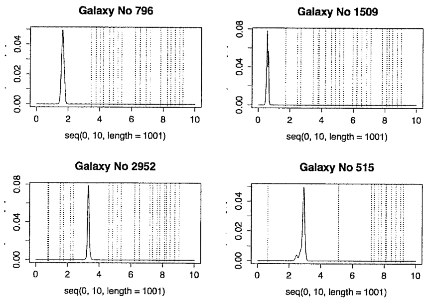
Figure 18: Some galaxies with one clear mode but the mode finding procedure couldn't pick out. Fortunately only a very small portion of galaxies(around 1%) have this behavior.
