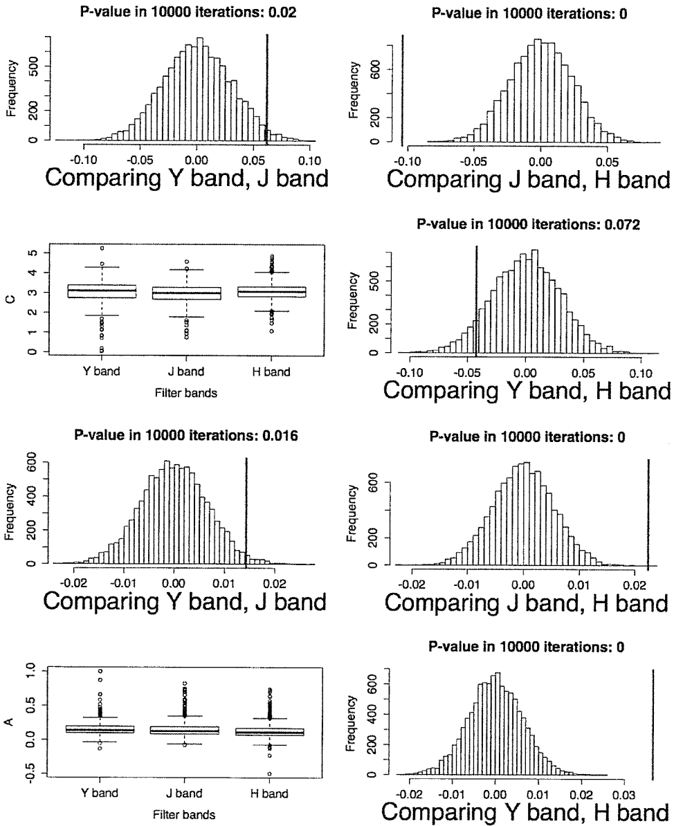
Figure 24: Bootstrap T test for C and A statistic in GOODS field. P-values are not adjusted for multiple testing.
