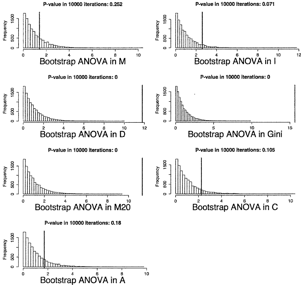
Figure 9: Bootstrap ANOVA for feature statistics in GOODSS field. The histogram is approximate null distribution of the test statistic. The red vertical line represent the statistic value calculated boowith the observed data.
