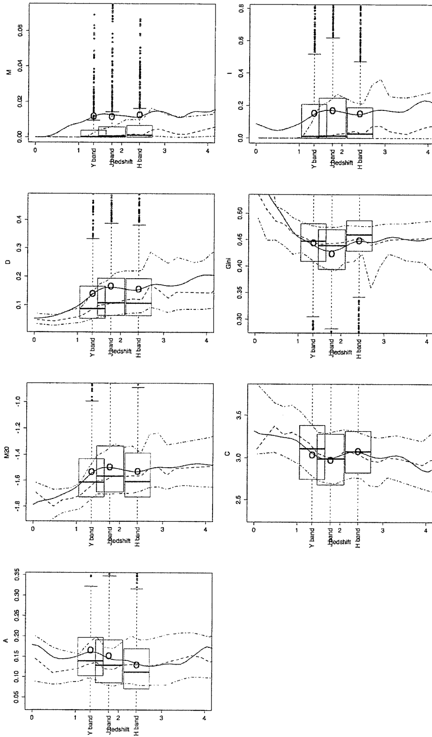
Figure 16: Same as Figure 12, but for GOODSN field using only data from Y, J and H band.
