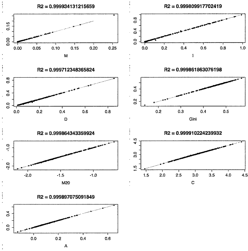
Figure 21: Comparing the weighted average from statistics taken in 3 filter bands to the true feature statistics taken in H band for galaxies in H band redshift range.
